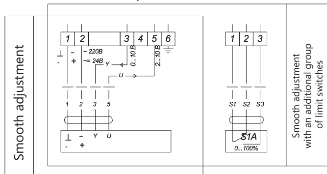
Stepless drive
