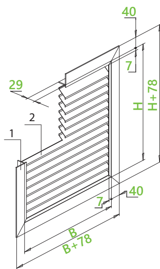
1 - casing; 2 - blade
