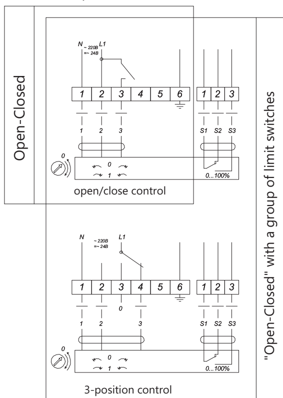
"Open-closed" drive
